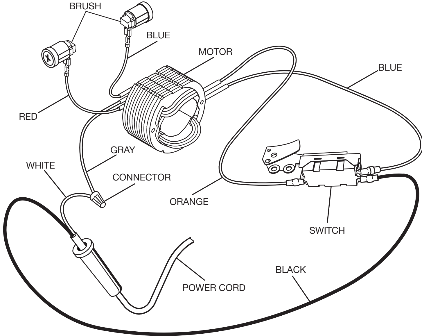
WIRING DIAGRAM
